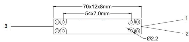
Slow axis working, Fast axis blocked Routing path is 3 to 1, 2(tap)
