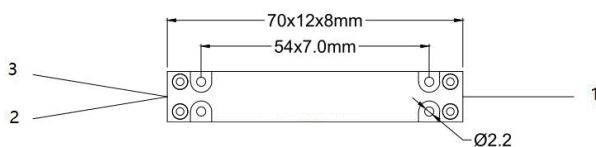
Both axis working Routing path is 3 to 1, 2(tap)
