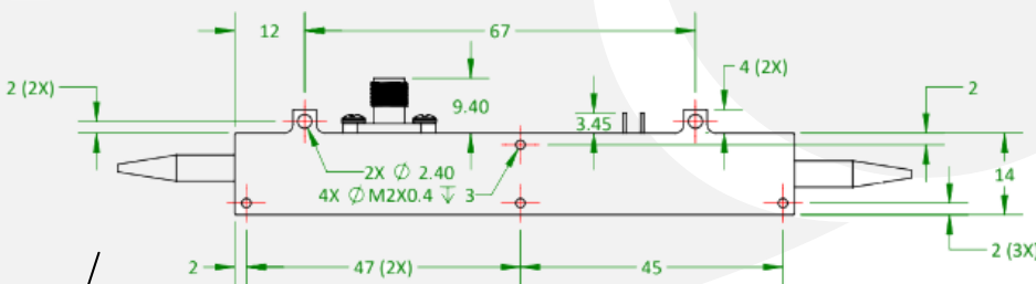
BOTTOM VIEW
